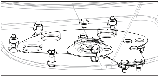
Complete Gate Assembly F50466
